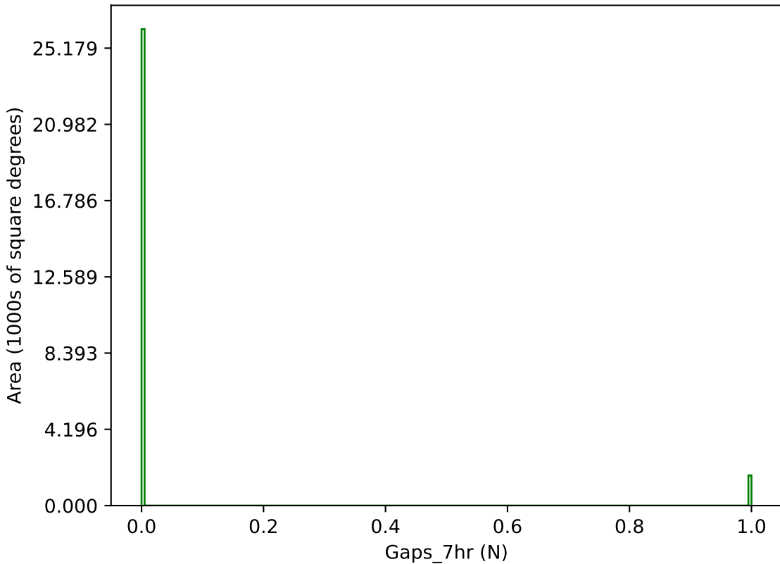
ddf_acor_sf25_lsf40_lsr50_v3.4_10yrs g band: Gaps_7hr
