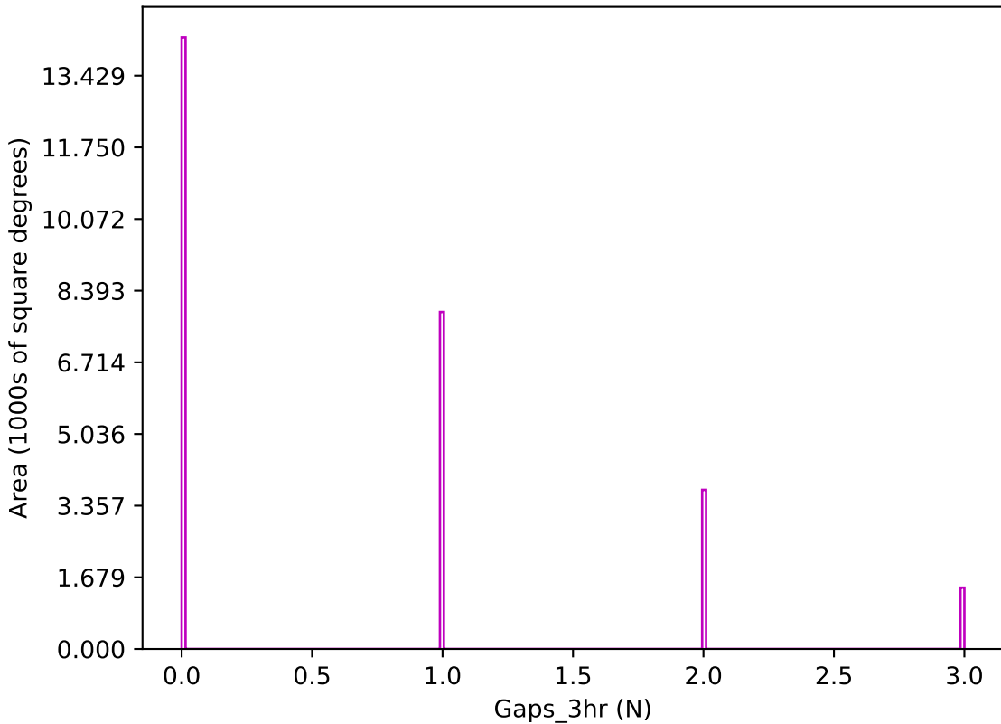
ddf_acor_sf25_lsf40_lsr50_v3.4_10yrs z band: Gaps_3hr
