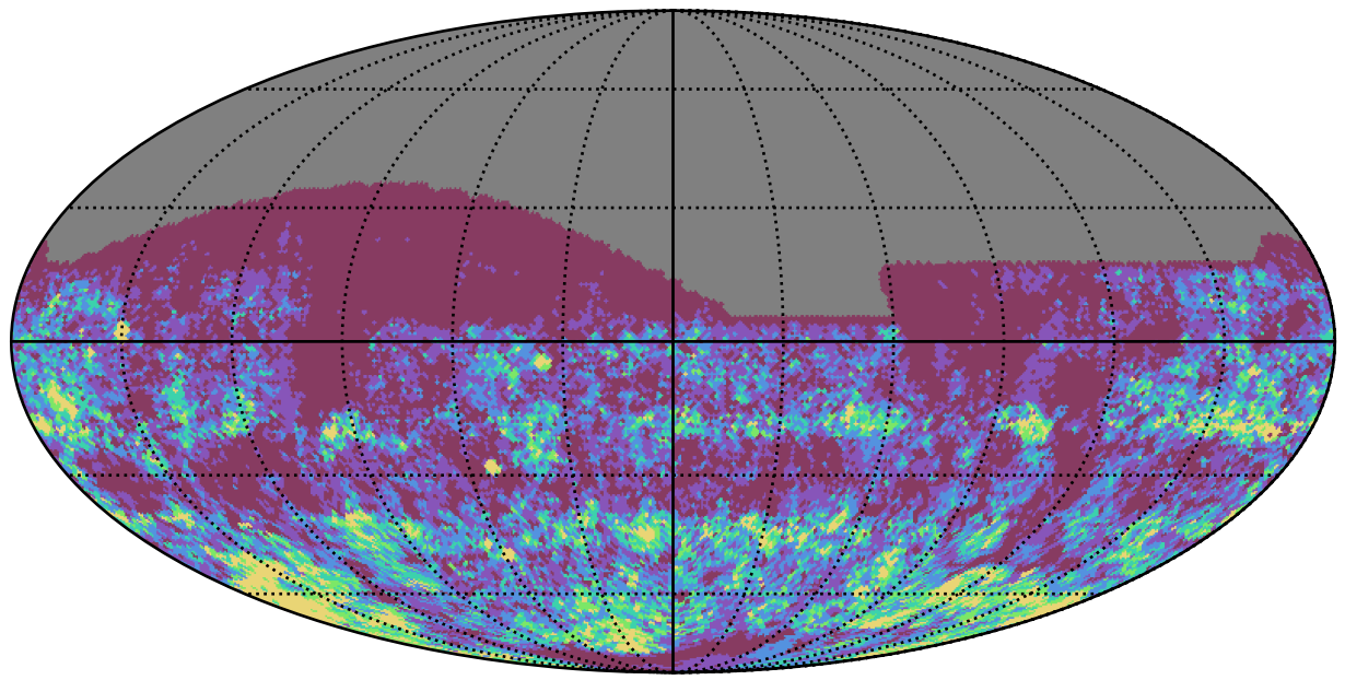
ddf_acor_sf25_lsf40_lsr50_v3.4_10yrs r band: Gaps_3hr
