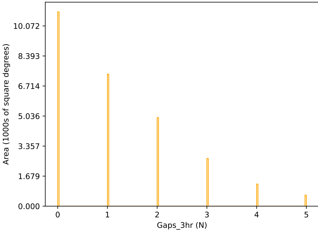
ddf_acor_sf25_lsf40_lsr50_v3.4_10yrs r band: Gaps_3hr
