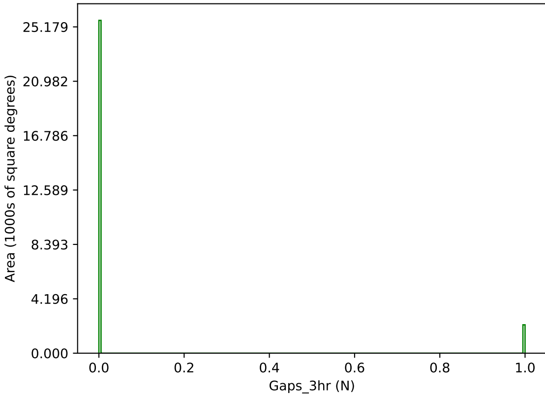
ddf_acor_sf25_lsf40_lsr50_v3.4_10yrs g band: Gaps_3hr
