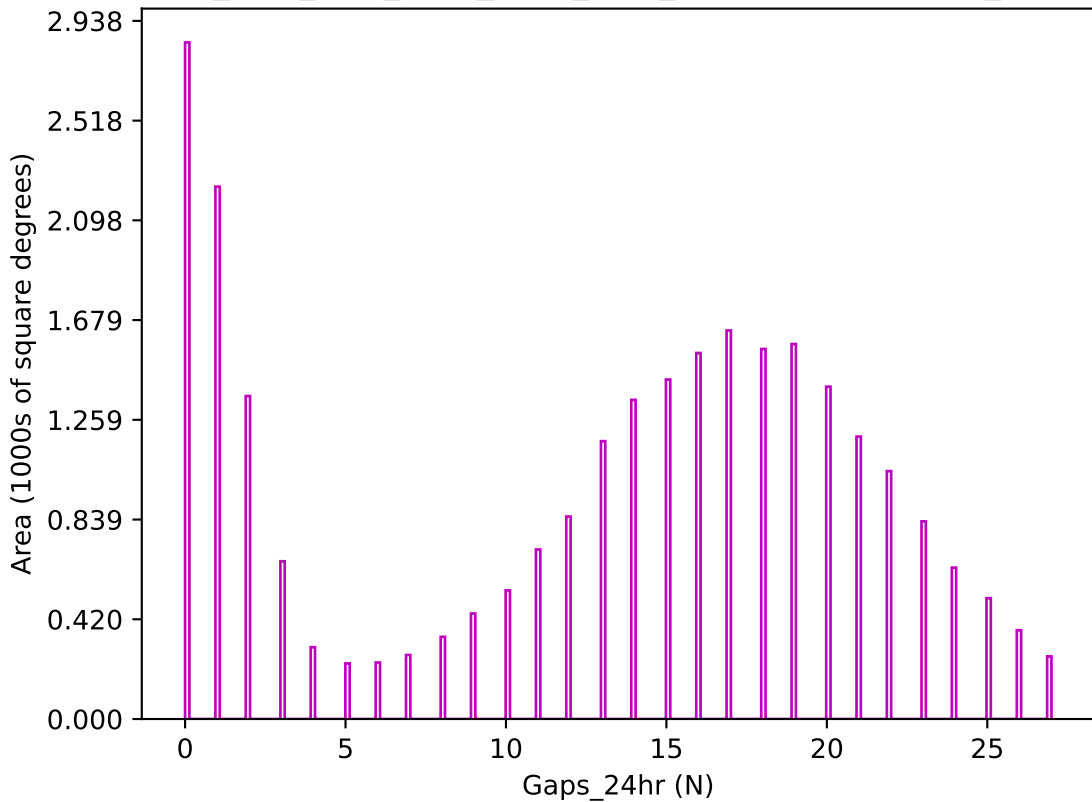
ddf_acor_sf25_lsf40_lsr50_v3.4_10yrs z band: Gaps_24hr
