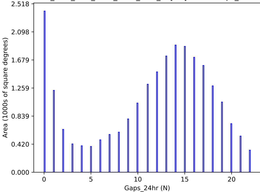
ddf_acor_sf25_lsf40_lsr50_v3.4_10yrs y band: Gaps_24hr
