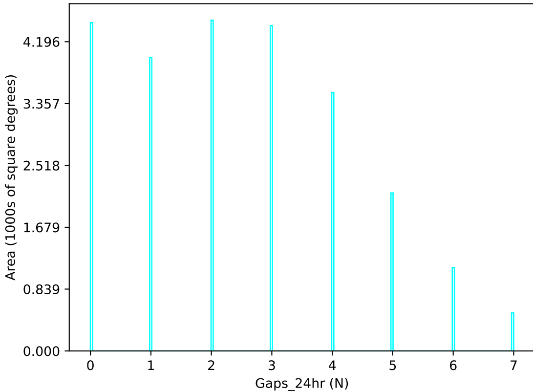
ddf_acor_sf25_lsf40_lsr50_v3.4_10yrs u band: Gaps_24hr
