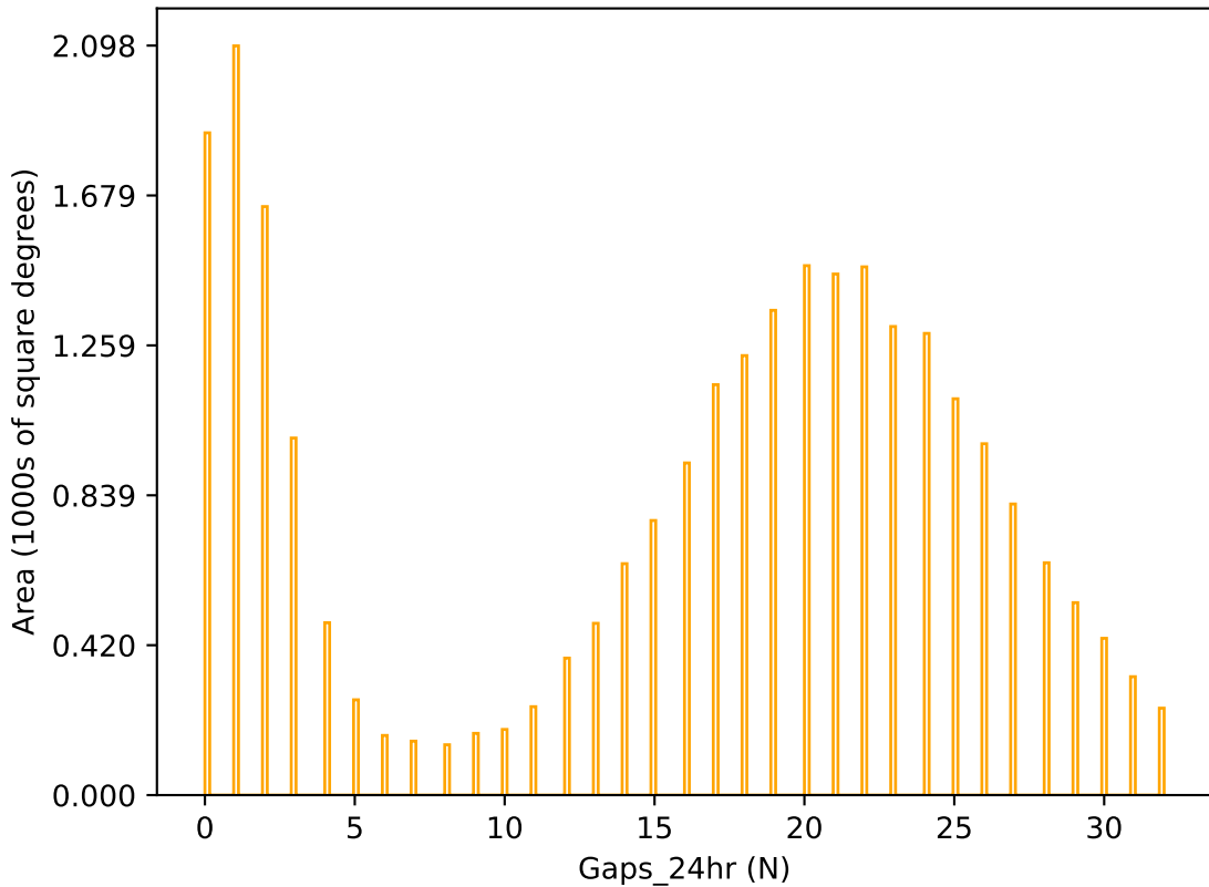
ddf_acor_sf25_lsf40_lsr50_v3.4_10yrs r band: Gaps_24hr
