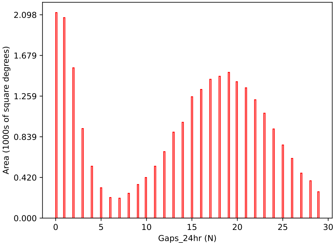
ddf_acor_sf25_lsf40_lsr50_v3.4_10yrs i band: Gaps_24hr
