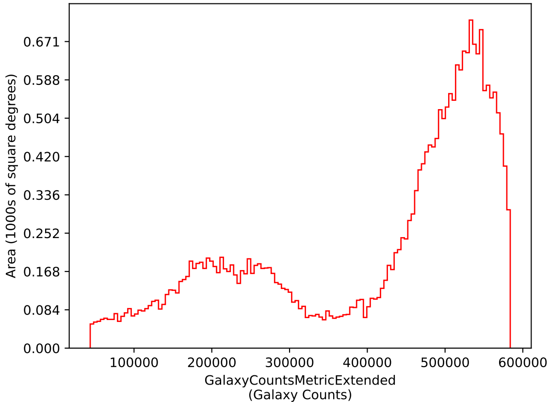
ddf_acor_sf25_ls40_lsr50_v3.4_10yrs i: GalaxyCountsMetricExtended
