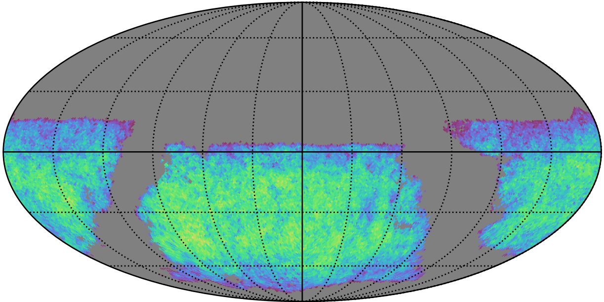
ddf_acor_sf25_lsf40_lsr50_v3.4_10yrs i band non-DD year 1: ExgalM5WithCuts
