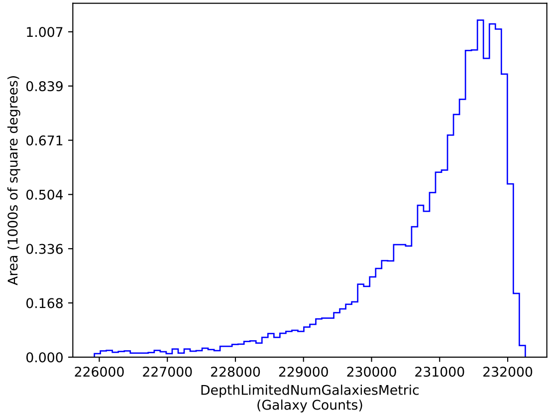
ddf_acor_sf25_lsf40_lsr50_v3.4_10yrs i band galaxies non-DD: DepthLimitedNumGalaxiesMetric
