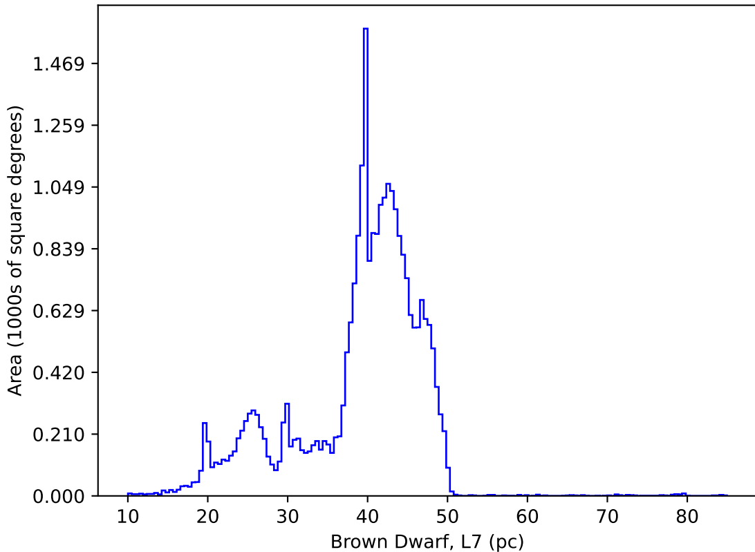
ddf_acor_sf25_lsf40_lsr50_v3.4_10yrs : Brown Dwarf, L7
