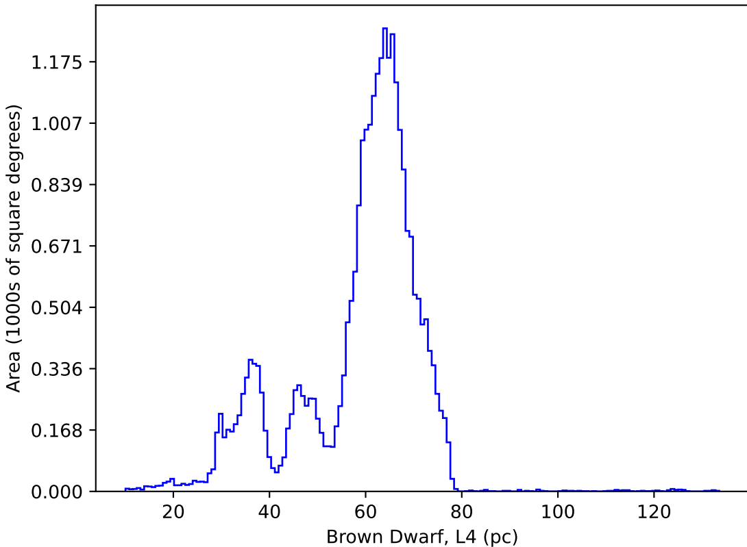
ddf_acor_sf25_lsf40_lsr50_v3.4_10yrs : Brown Dwarf, L4
