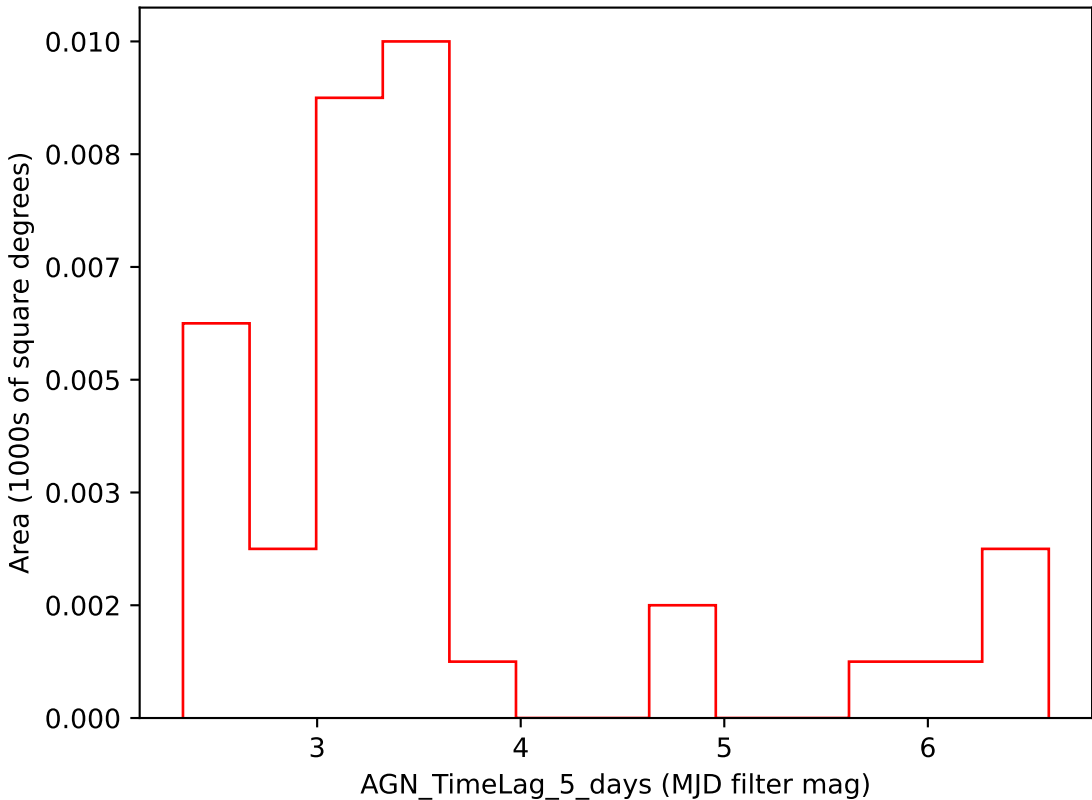
ddf_acor_sf25_lsf40_lsr50_v3.4_10yrs i band: AGN_TimeLag_5_days
