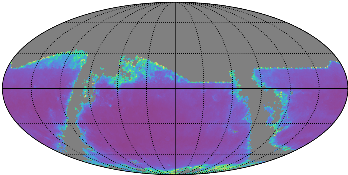
ddf_acor_sf25_lsf40_lsr50_v3.4_10yrs r band: AGN SF_uncert
