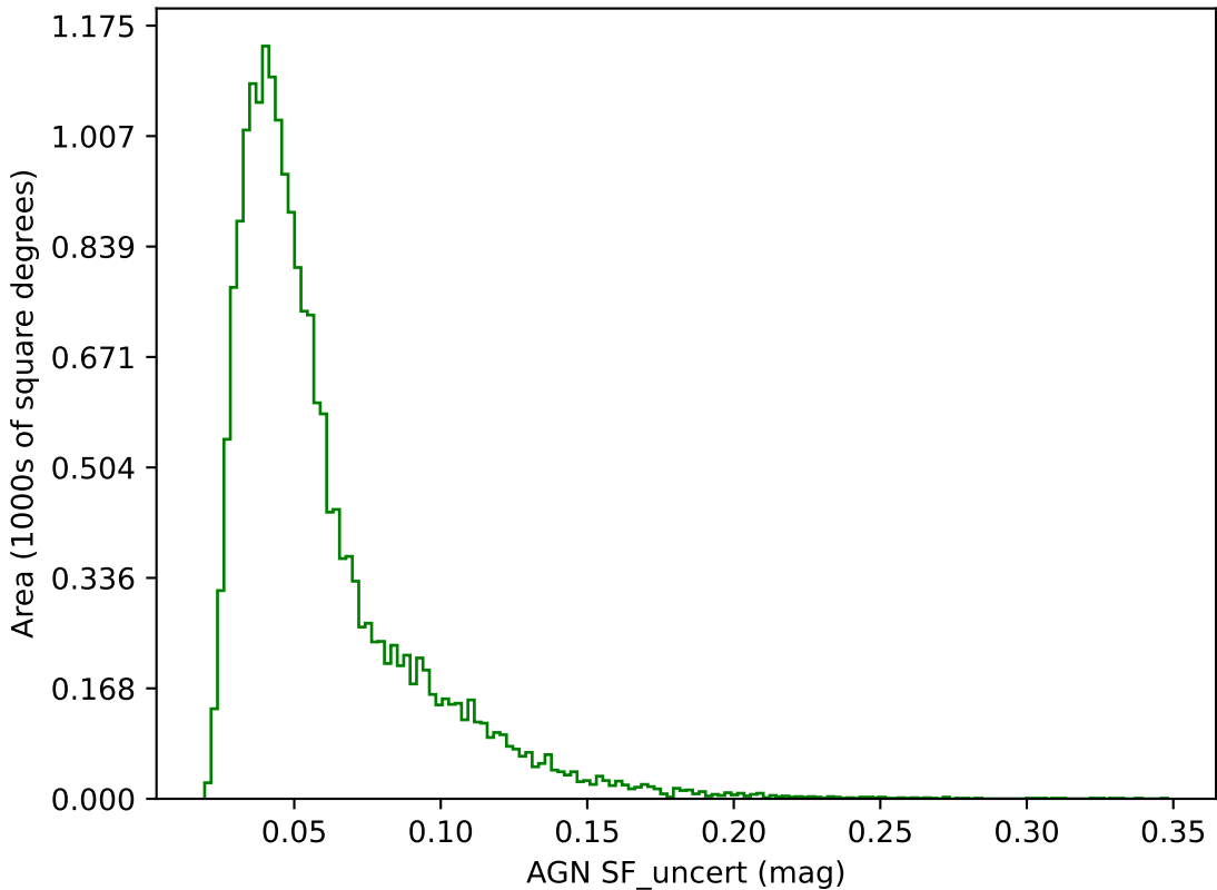
ddf_acor_sf25_lsf40_lsr50_v3.4_10yrs g band: AGN SF_uncert
