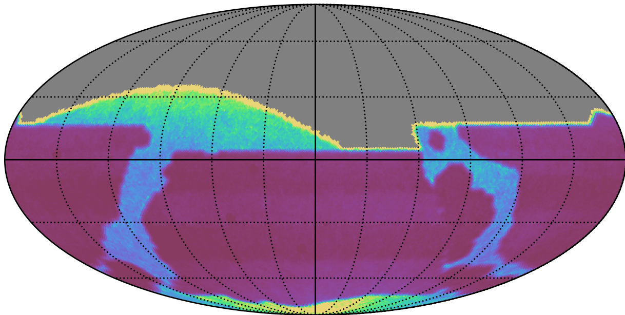
ddf_acor_sf25_lsf40_lsr50_v3.4_10yrs : properMotion
