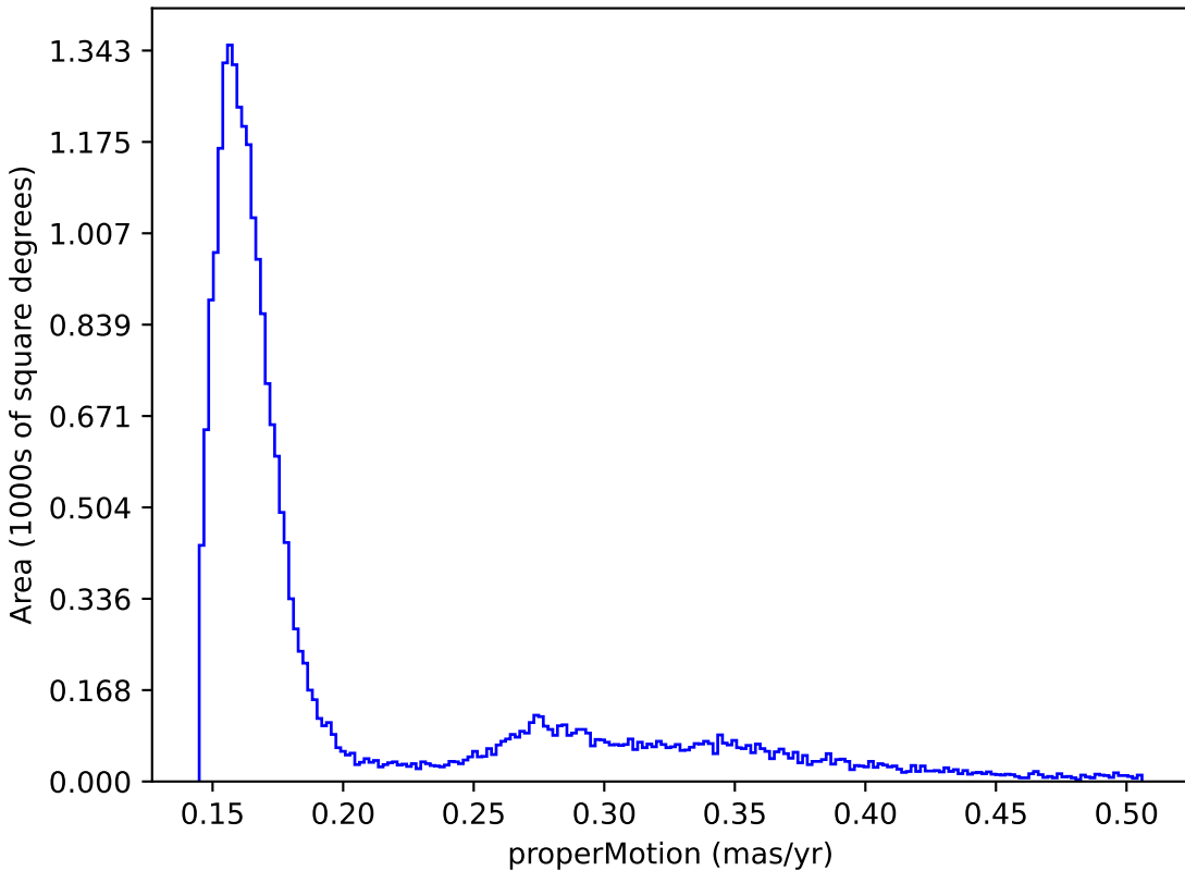
ddf_acor_sf25_lsf40_lsr50_v3.4_10yrs : properMotion
