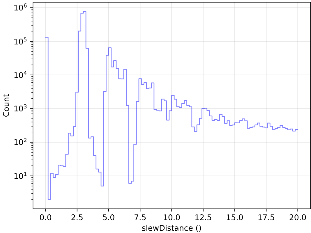
ddf_acor_sf25_lsf40_lsr50_v3.4_10yrs All visits: Zoom Slew Distance Histogram
