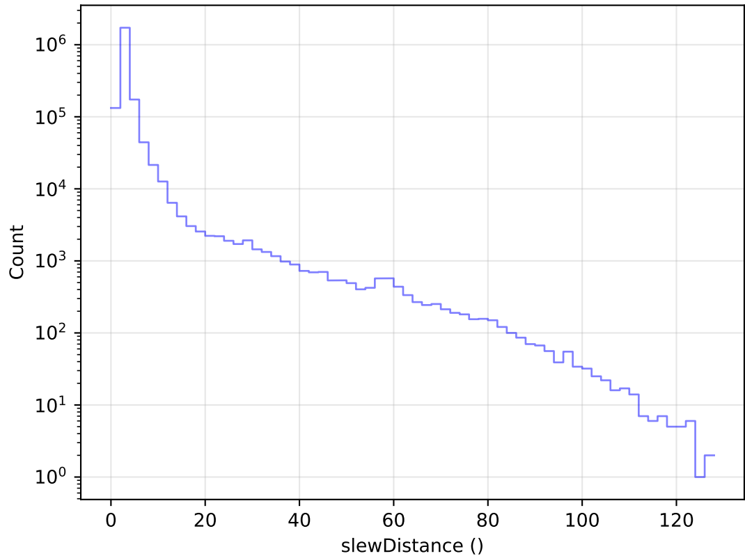
ddf_acor_sf25_lsf40_lsr50_v3.4_10yrs All visits: Slew Distance Histogram
