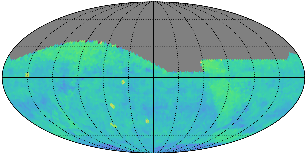
ddf_acor_sf25_lsf40_lsr50_v3.4_10yrs (g or r or i): PairFraction
