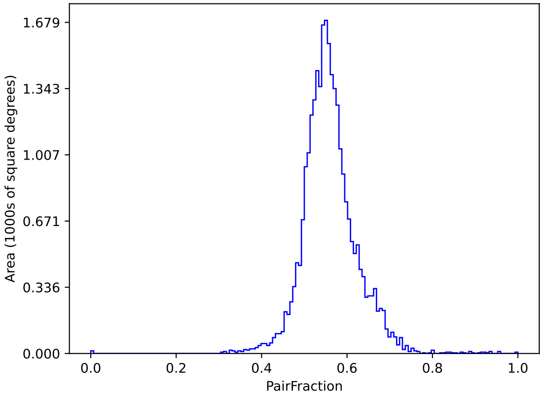
ddf_acor_sf25_lsf40_lsr50_v3.4_10yrs (g or r or i): PairFraction
