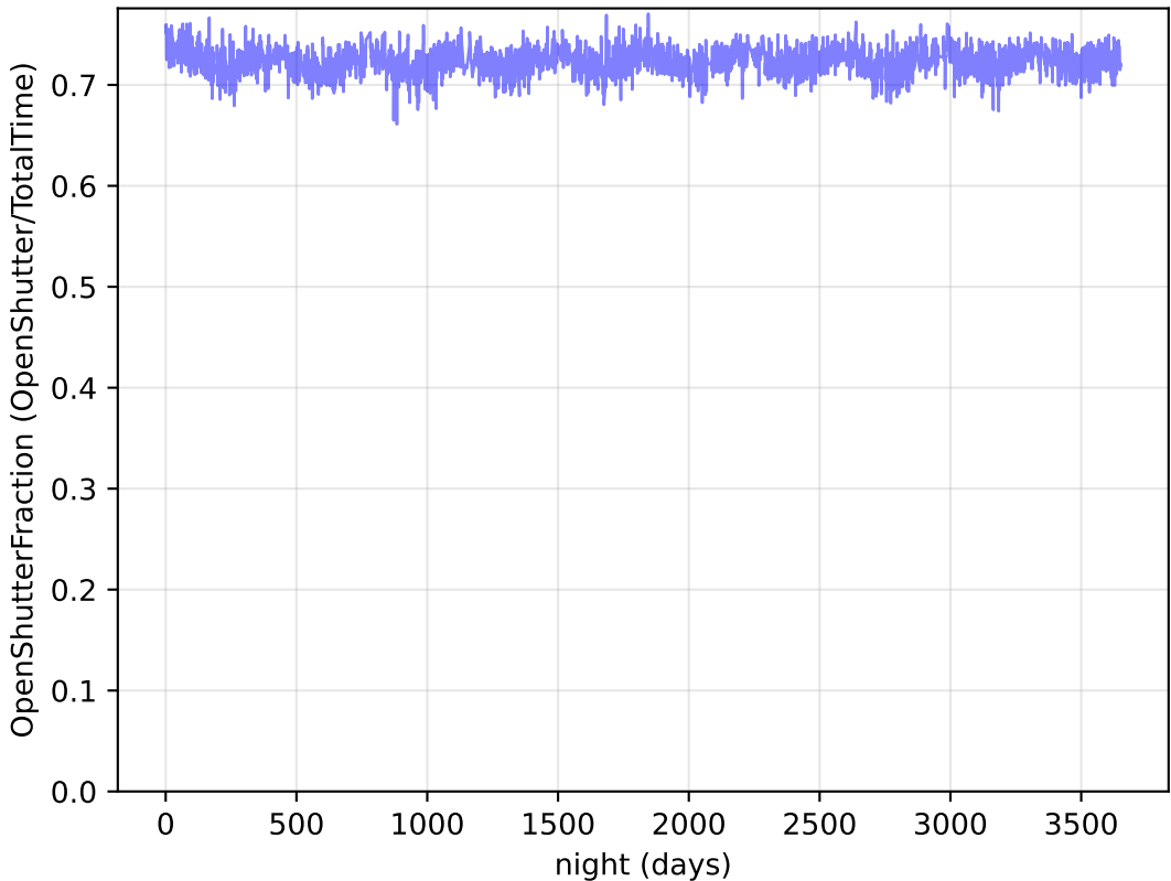
ddf_acor_sf25_lsf40_lsr50_v3.4_10yrs : OpenShutterFraction
