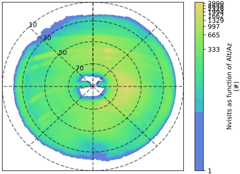
ddf_acor_sf25_lsf40_lsr50_v3.4_10yrs z: Nvisits as function of Alt/Az
