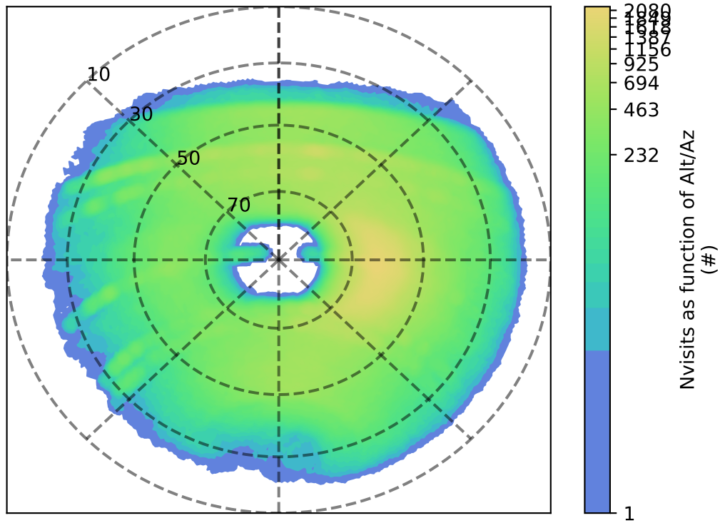
ddf_acor_sf25_lsf40_lsr50_v3.4_10yrs y: Nvisits as function of Alt/Az
