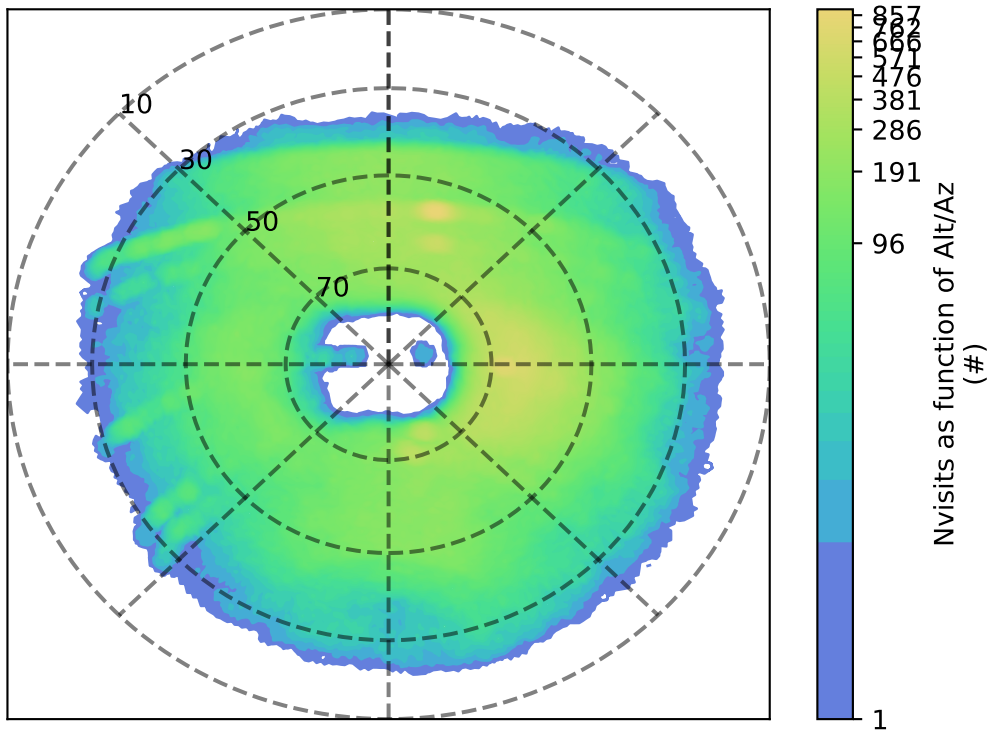
ddf_acor_sf25_lsf40_lsr50_v3.4_10yrs u: Nvisits as function of Alt/Az
