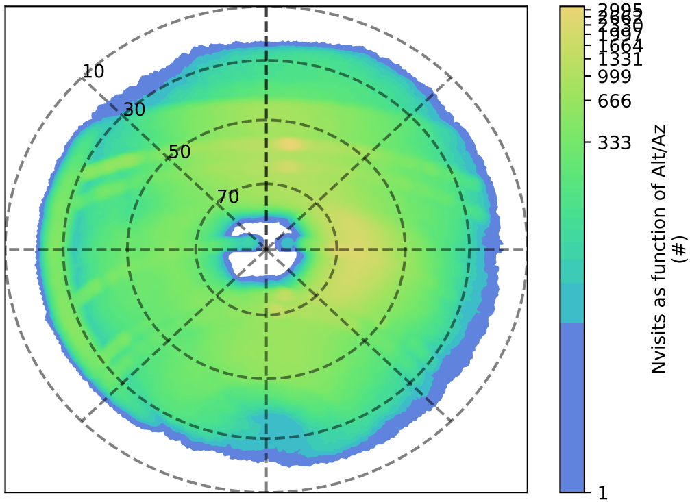
ddf_acor_sf25_lsf40_lsr50_v3.4_10yrs r: Nvisits as function of Alt/Az
