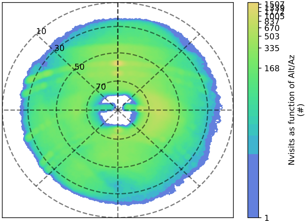
ddf_acor_sf25_lsf40_lsr50_v3.4_10yrs g: Nvisits as function of Alt/Az
