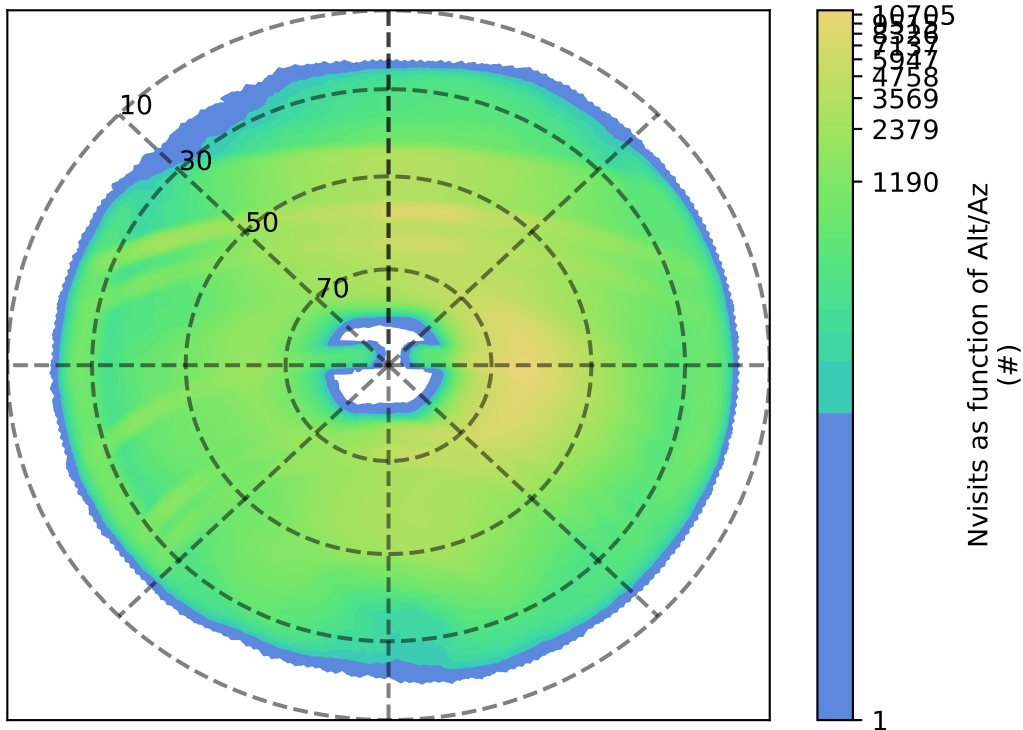
ddf_acor_sf25_lsf40_lsr50_v3.4_10yrs : Nvisits as function of Alt/Az
