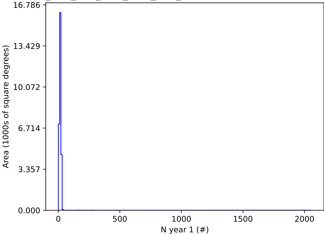
ddf_acor_sf25_lsf40_lsr50_v3.4_10yrs r and night < 365: N year 1
