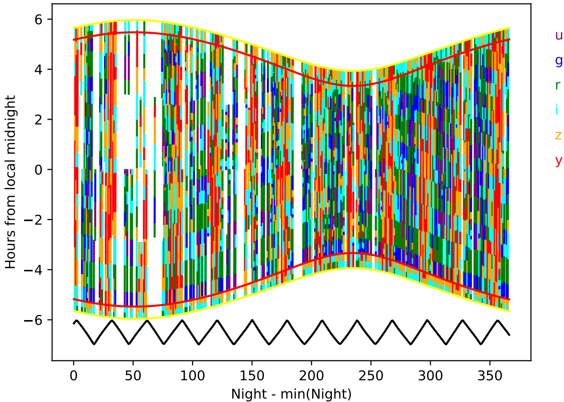
ddf_acor_sf25_lsf40_lsr50_v3.4_10yrs year 9-10: Hourglass
