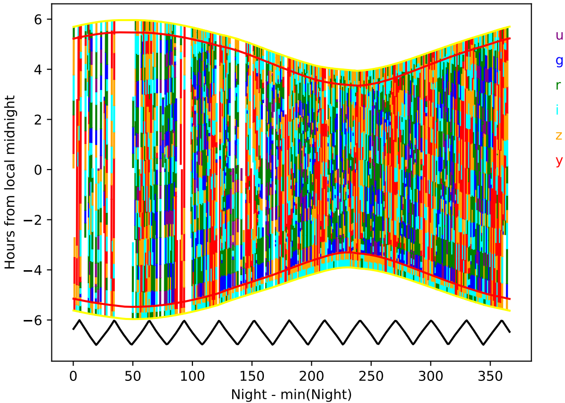
ddf_acor_sf25_lsf40_lsr50_v3.4_10yrs year 6-7: Hourglass
