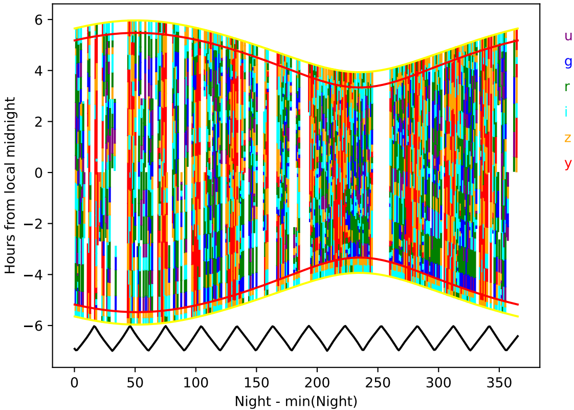
ddf_acor_sf25_lsf40_lsr50_v3.4_10yrs year 5-6: Hourglass
