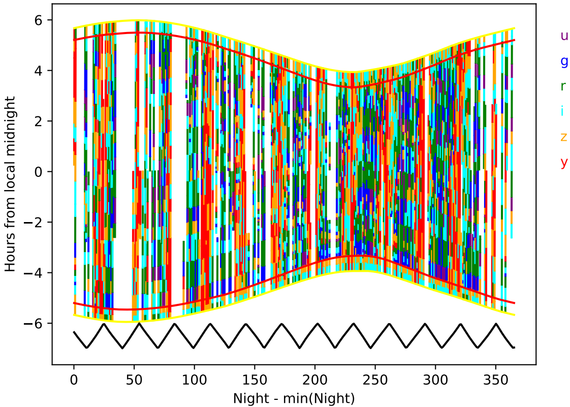
ddf_acor_sf25_lsf40_lsr50_v3.4_10yrs year 4-5: Hourglass
