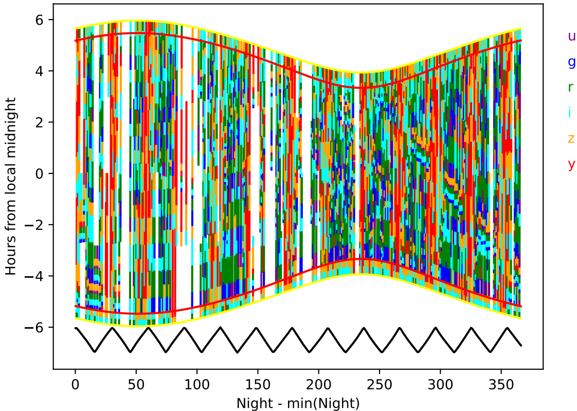
ddf_acor_sf25_lsf40_lsr50_v3.4_10yrs year 1-2: Hourglass
