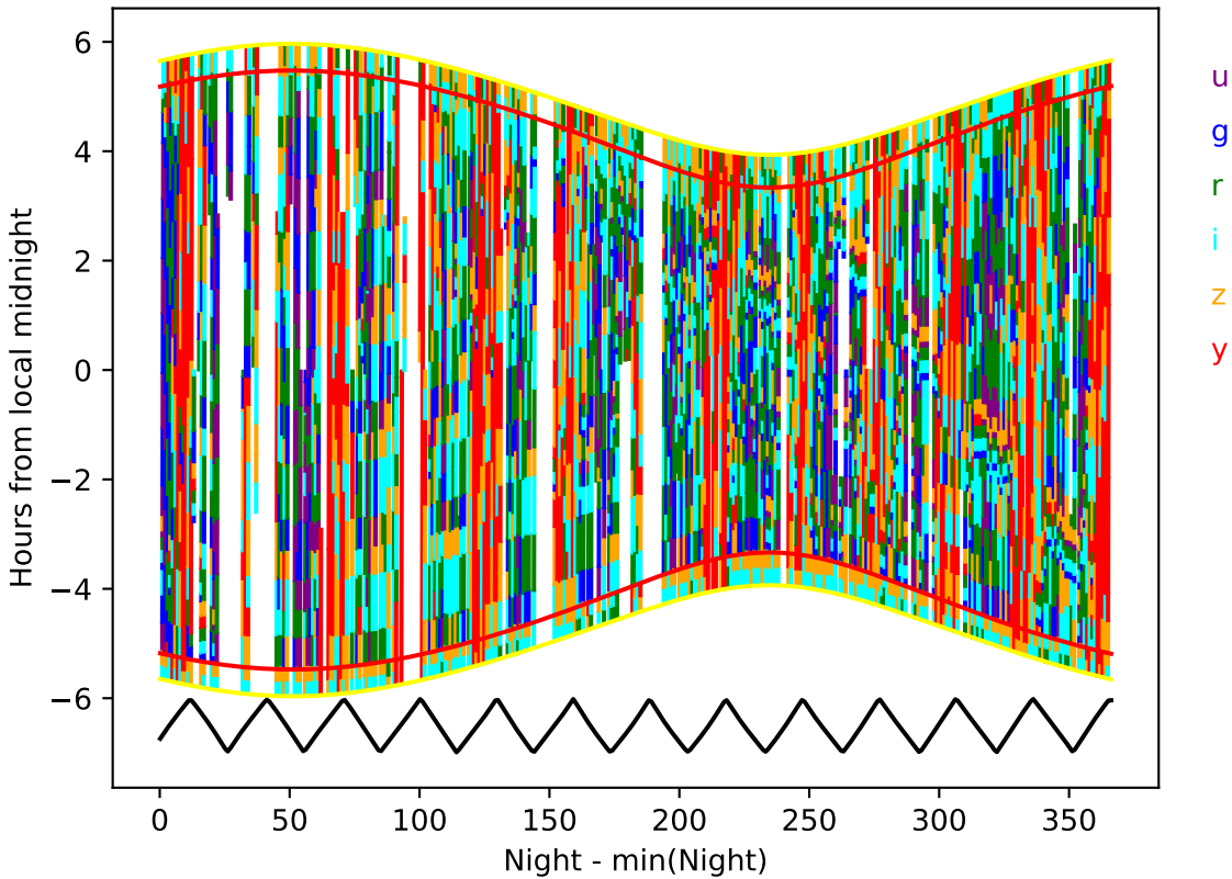
ddf_acor_sf25_lsf40_lsr50_v3.4_10yrs year 0-1: Hourglass
