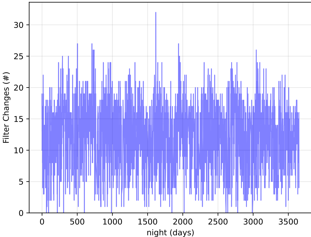
ddf_acor_sf25_lsf40_lsr50_v3.4_10yrs : Filter Changes
