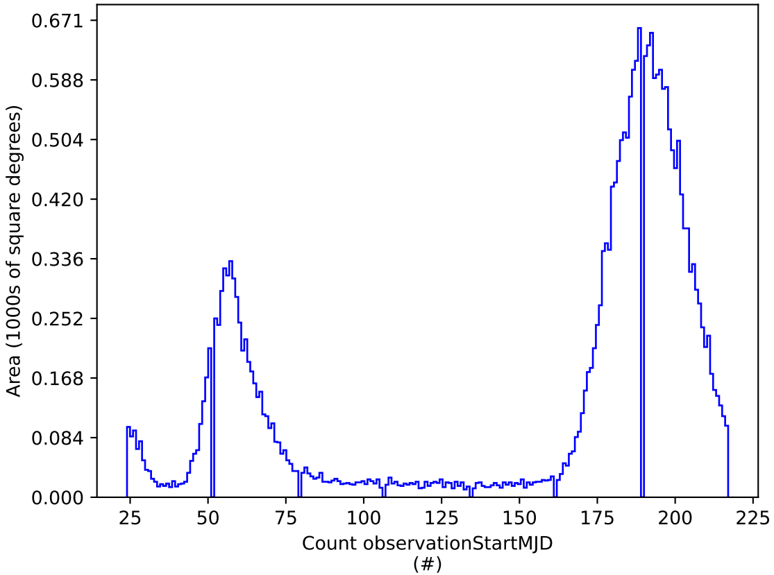
ddf_acor_sf25_lsf40_lsr50_v3.4_10yrs i: Count observationStartMJD
