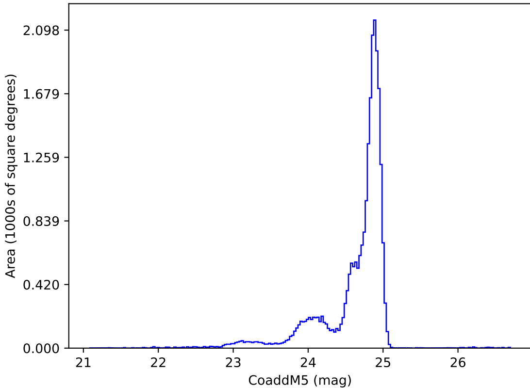
ddf_acor_sf25_lsf40_lsr50_v3.4_10yrs y: CoaddM5
