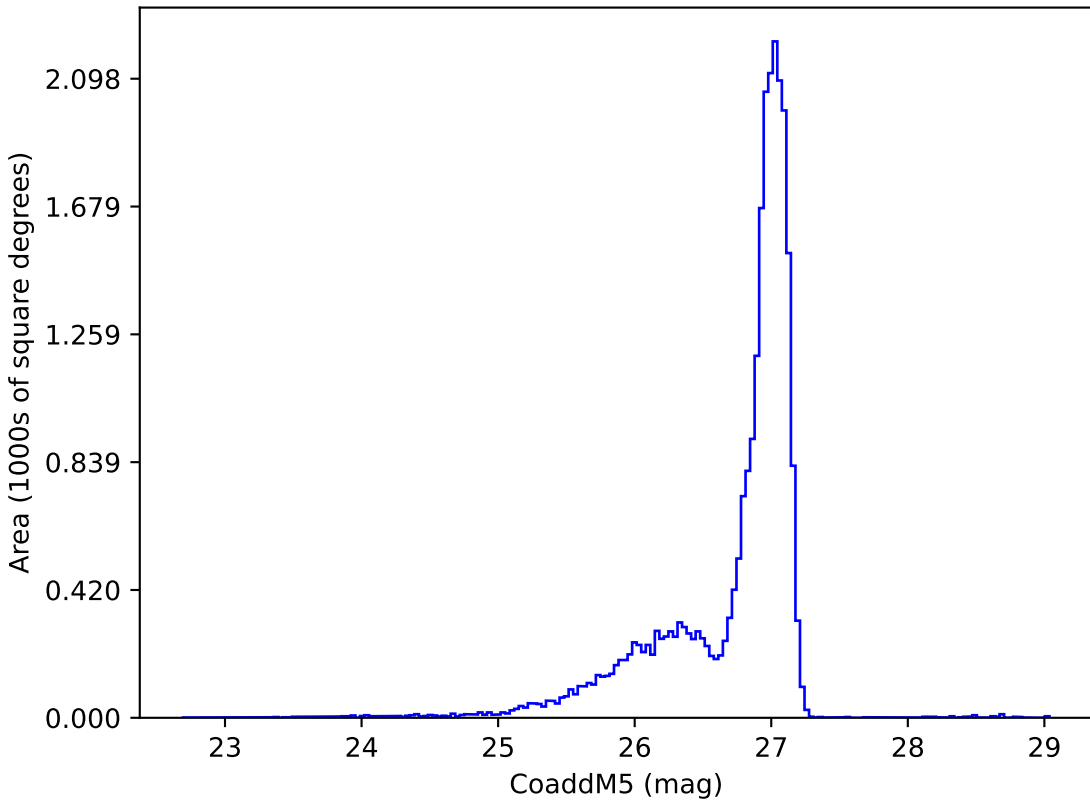
ddf_acor_sf25_lsf40_lsr50_v3.4_10yrs r: CoaddM5
