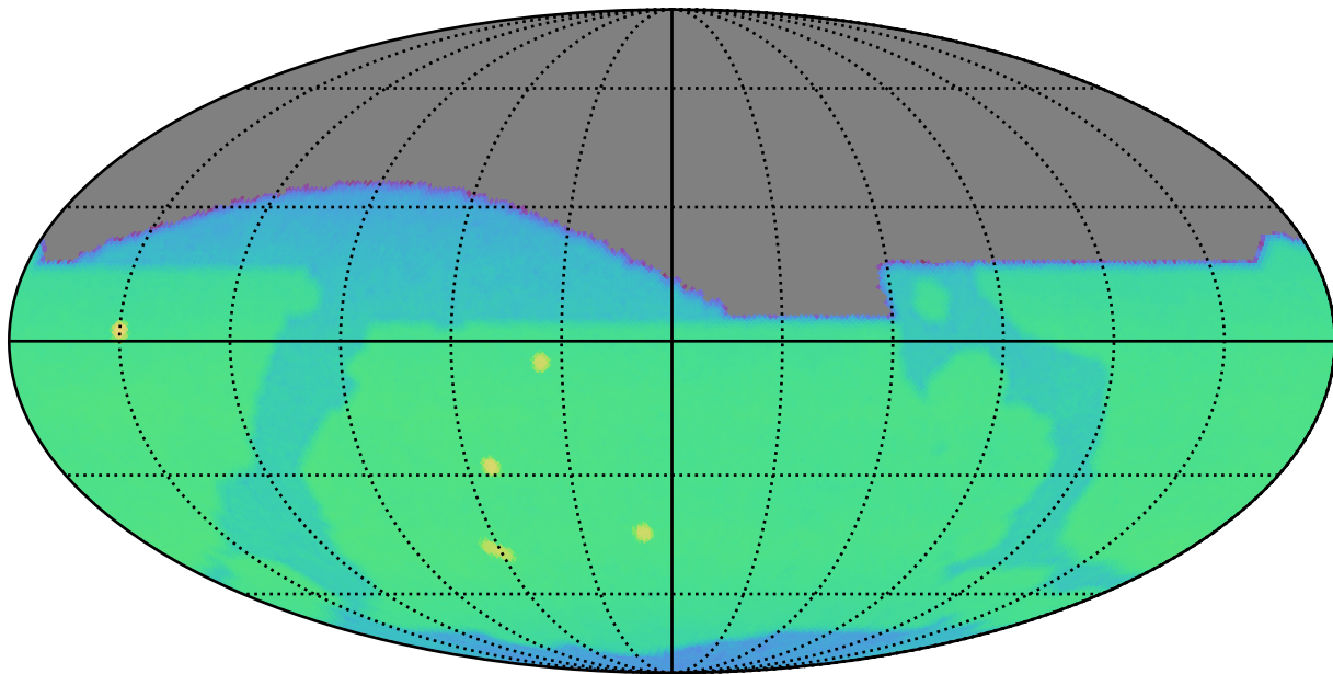
ddf_acor_sf25_lsf40_lsr50_v3.4_10yrs i: CoaddM5
