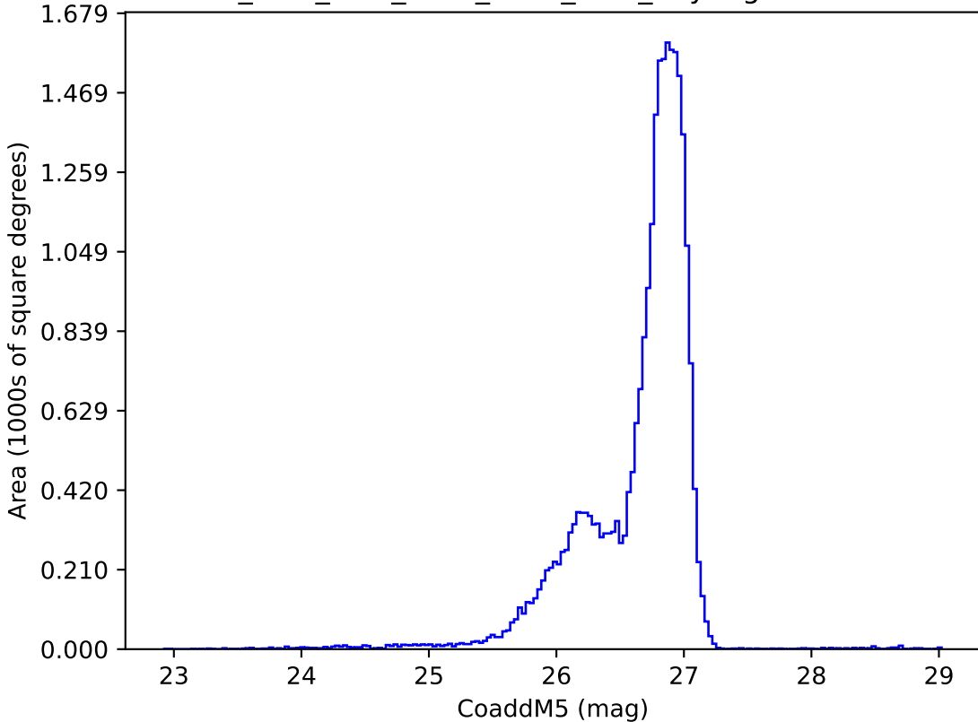
ddf_acor_sf25_lsf40_lsr50_v3.4_10yrs g: CoaddM5
