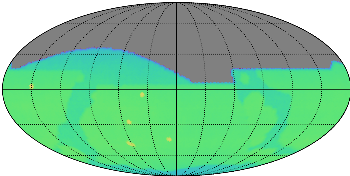
ddf_acor_sf25_lsf40_lsr50_v3.4_10yrs : CoaddM5
