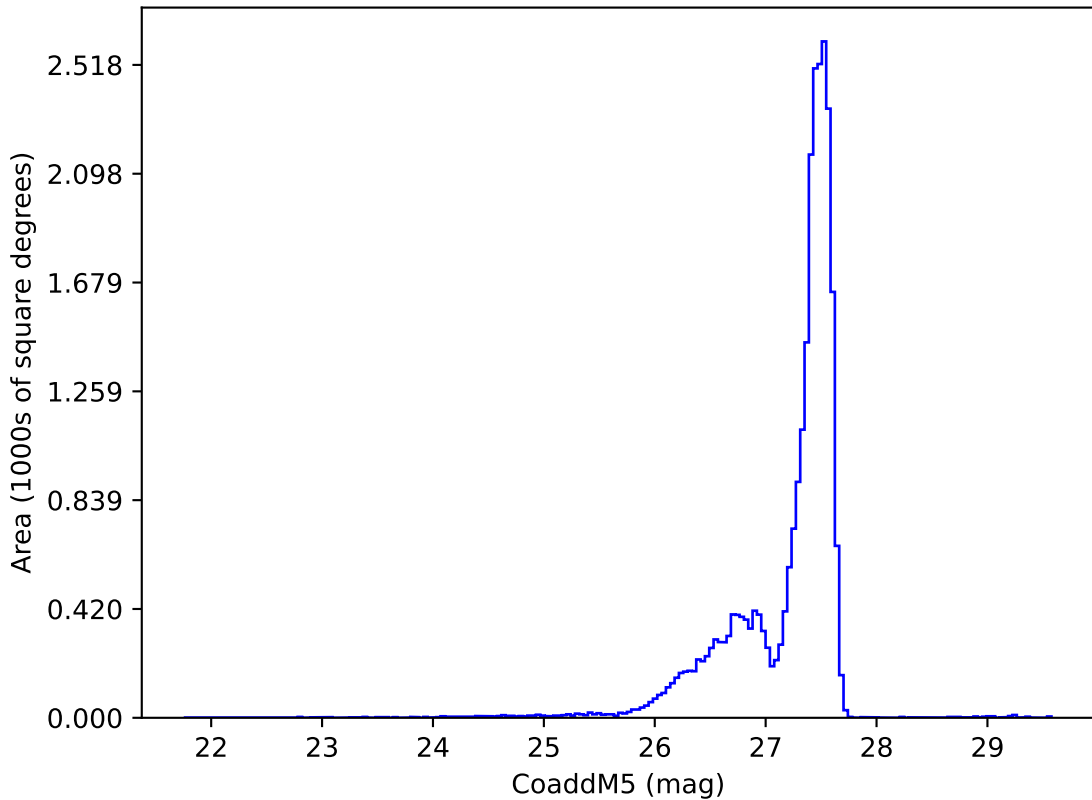
ddf_acor_sf25_lsf40_lsr50_v3.4_10yrs : CoaddM5
