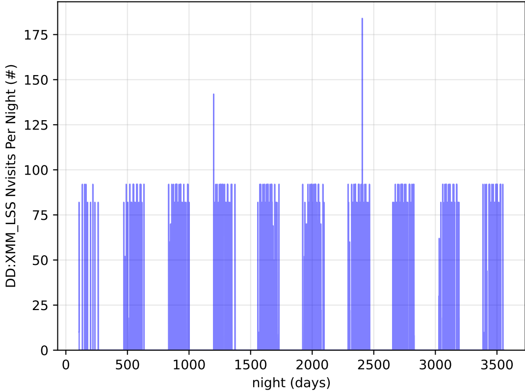
ddf_acor_sf25_lsf40_lsr50_v3.4_10yrs all bands: DD:XMM_LSS Nvisits Per Night
