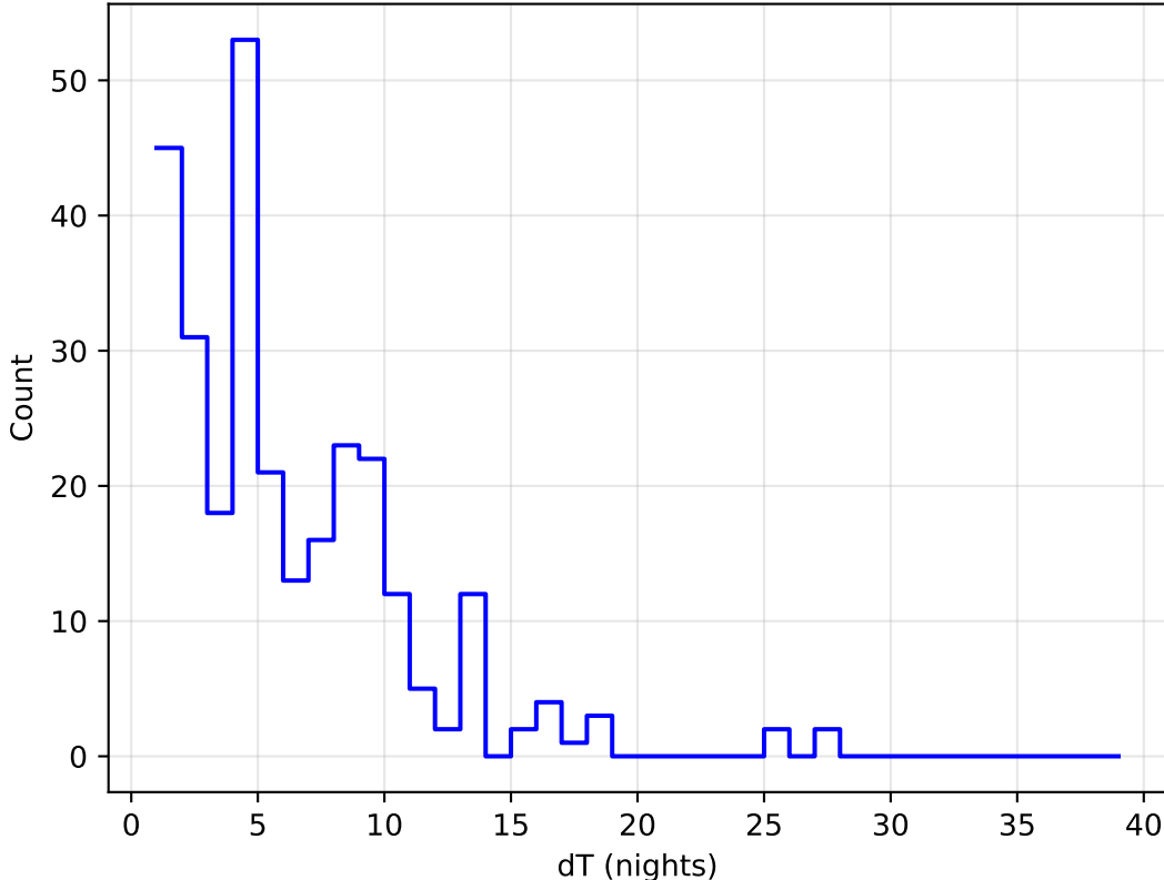
ddf_acor_sf25_lsf40_lsr50_v3.4_10yrs all bands: DD:XMM_LSS Delta Nights Histogram
