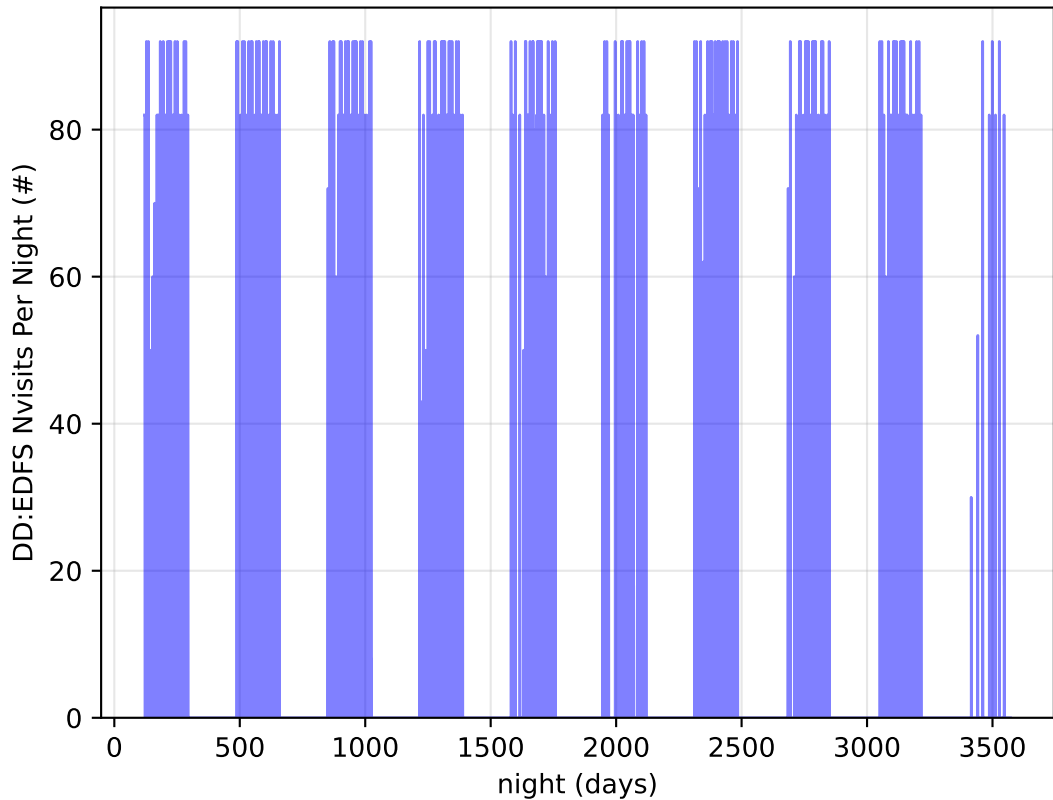
ddf_acor_sf25_lsf40_lsr50_v3.4_10yrs all bands: DD:EDFS Nvisits Per Night
