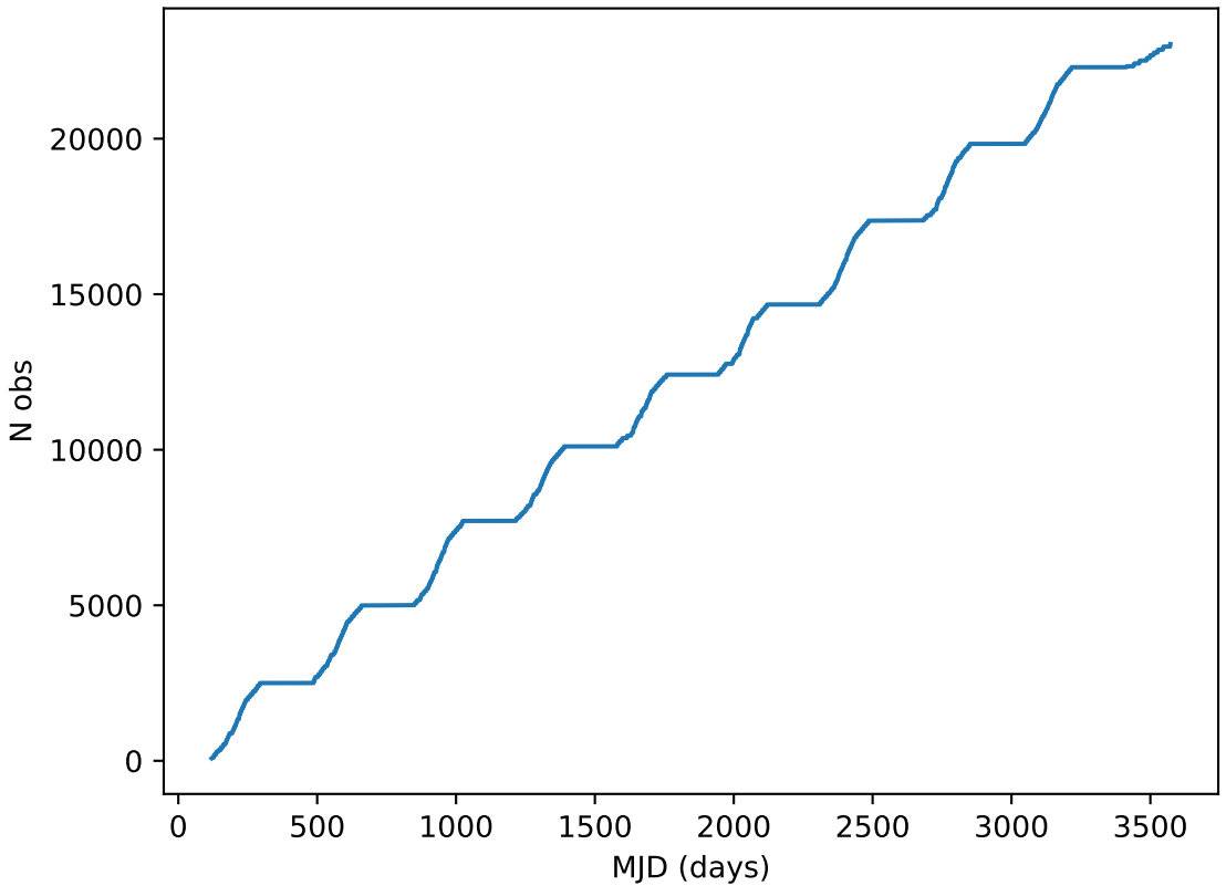
ddf_acor_sf25_lsf40_lsr50_v3.4_10yrs all bands: DD:EDFS Cumulative NVisits
